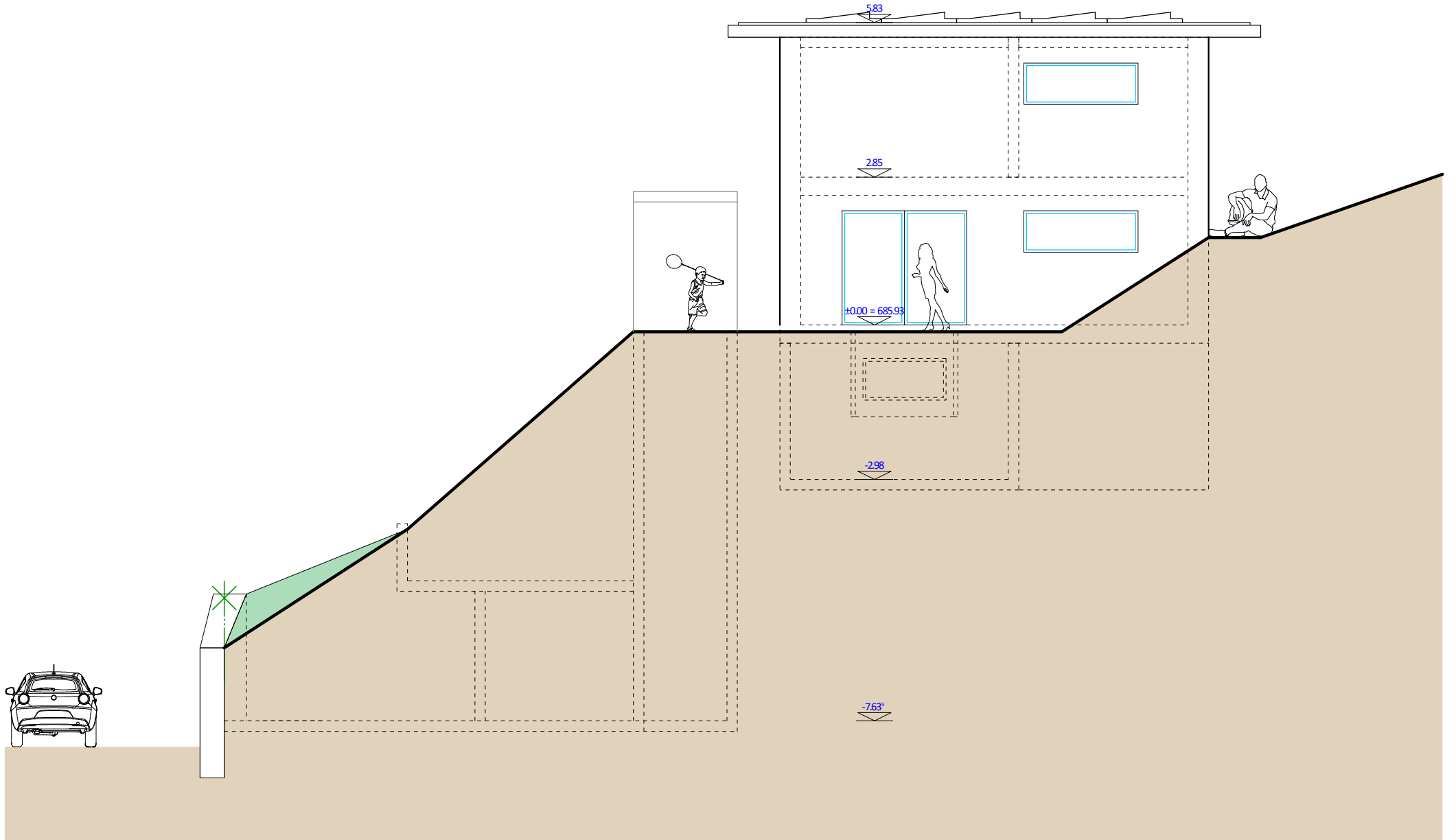
0 1 2 3 5 ECH. 1:100 FACADE NE - VILLA A
