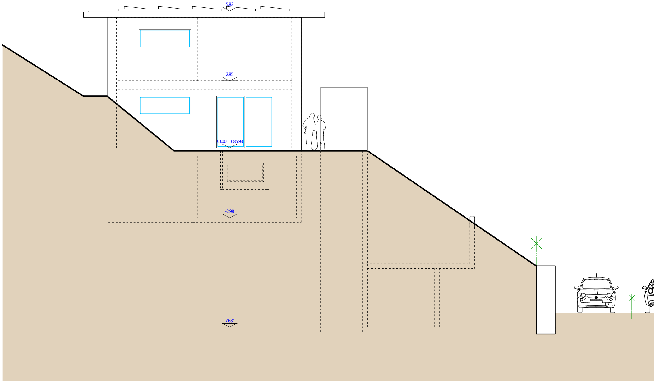
0 1 2 3 5 ECH. 1:100 FACADE SO - VILLA B
